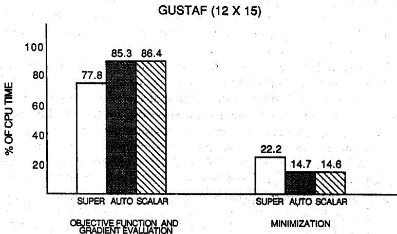
Fig. 5. Histograms of the relative percentages of scalar, automatic vectorization, and super (manual) vectorization code given as percentages of total CPU time spent in minimization code (GUSTAF problem, 12 \times 15 mesh).
