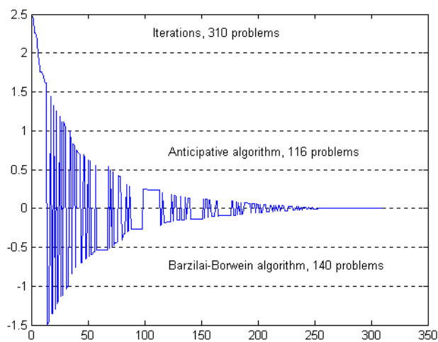
Fig. 3. Iterations, 310 problems
