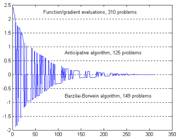
Fig. 2. Function/gradient evaluations, 310 problems
