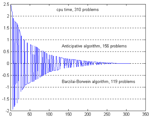
Fig. 1. CPU performance profile. 310 problems
